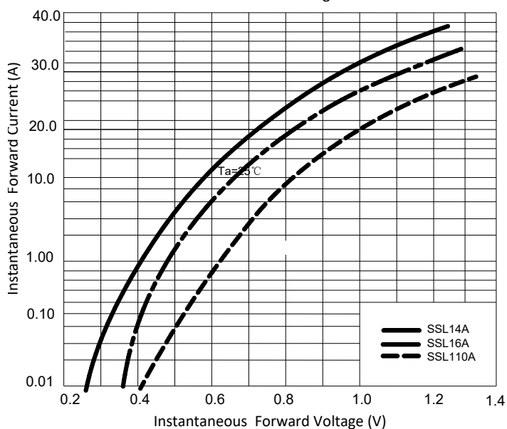
FIG3: Forward Voltage
